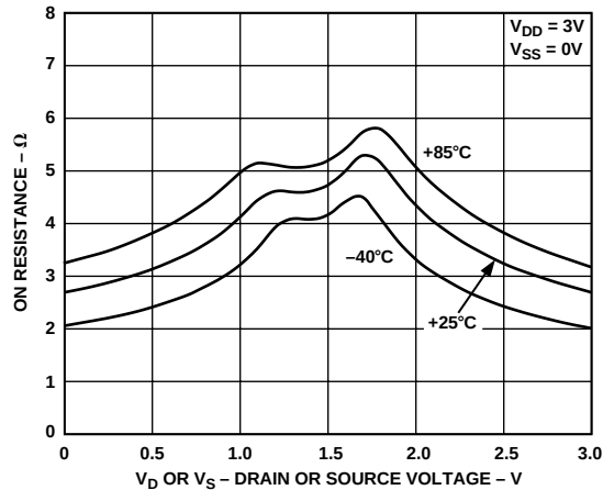
Figure 4. On Resistance as a Function of V_D ( V_S ) for Different Temperatures, Single Supply
