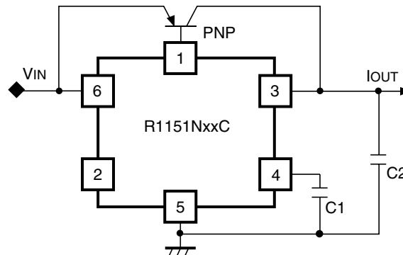
Fig.2 Supply Current Test Circuit C1=220pF , C2=10\mu F
