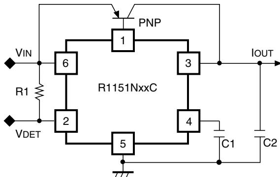
Fig.1 Standard test Circuit R1=470k\Omega C1=220pF , C2=10\mu F
