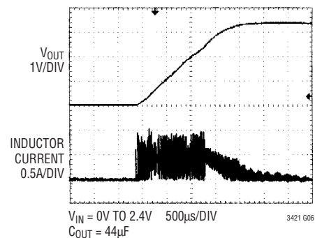
Inrush Current Control
