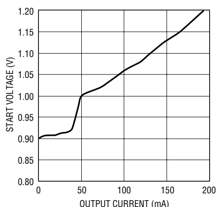
Start-Up Voltage vs Output Current
