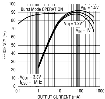
Single Cell to 3.3V Efficiency
