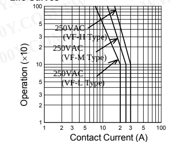
Life Curves
