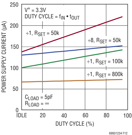
Figure 12. I_{S(ACTIVE)} vs Output Duty Cycle
