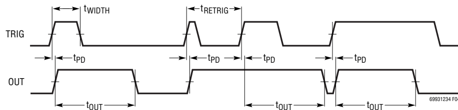
Figure 4. Retriggering Timing Diagram (LTC6993-2, POL = 0)
