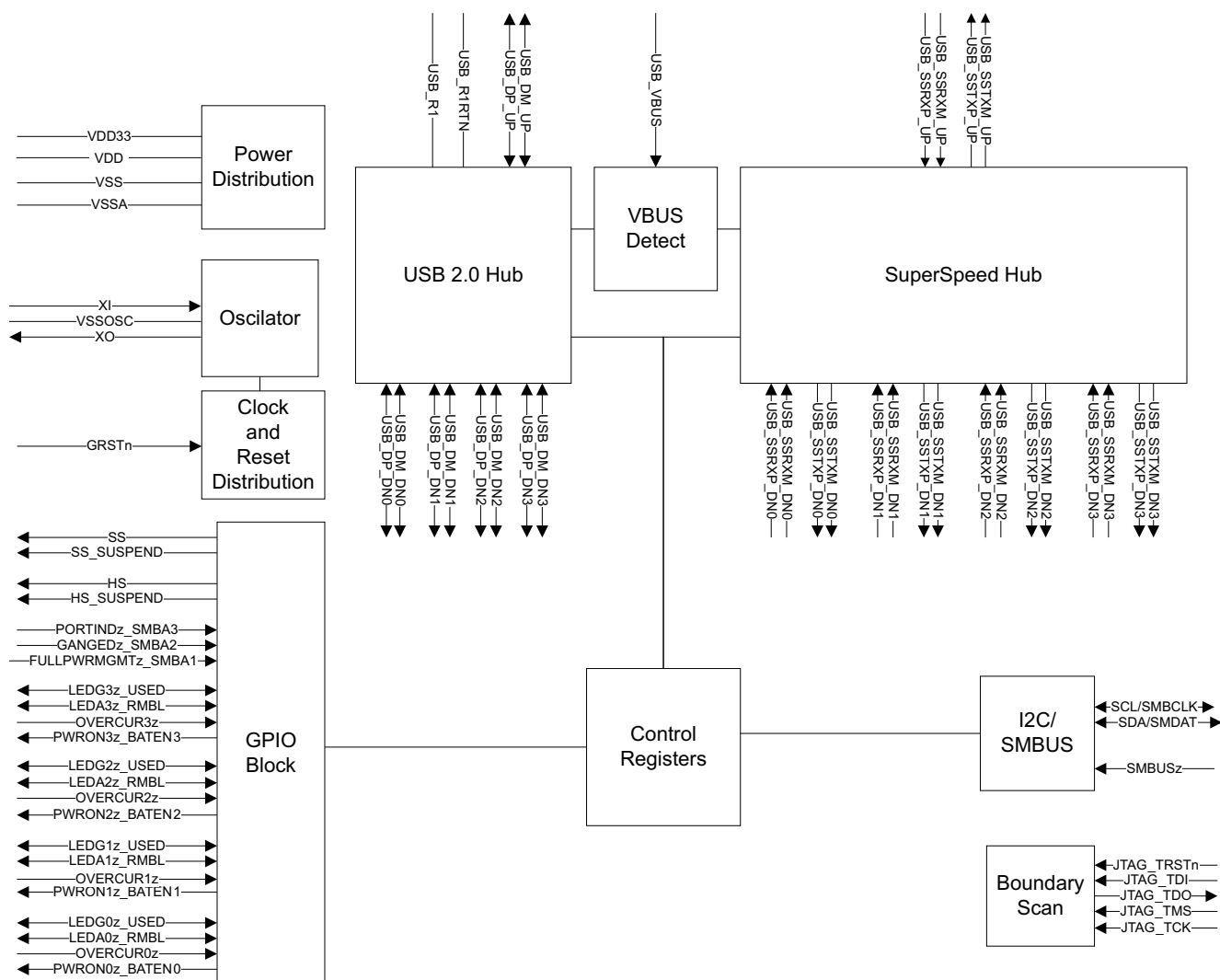
Figure 1-2. TUSB8040A1 Functional Block Diagram
