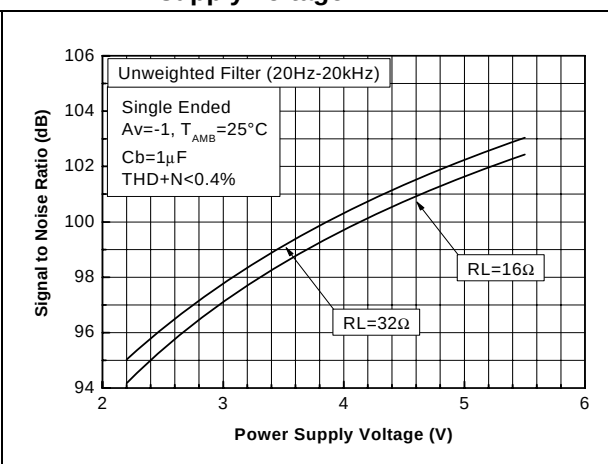
Figure 55. Signal to noise ratio vs. power supply voltage
