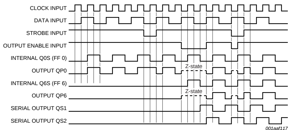
Fig 6. Timing diagram
