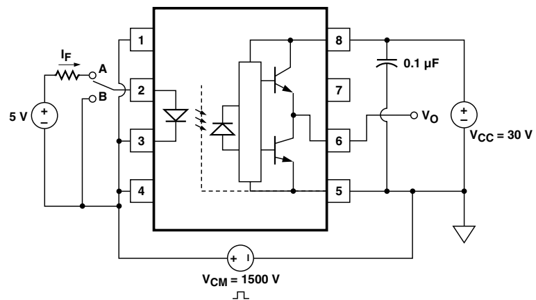
Figure 18. CMR Test Circuit and Waveforms.
