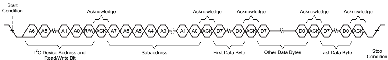
Figure 28. Multiple-Byte Write Transfer
