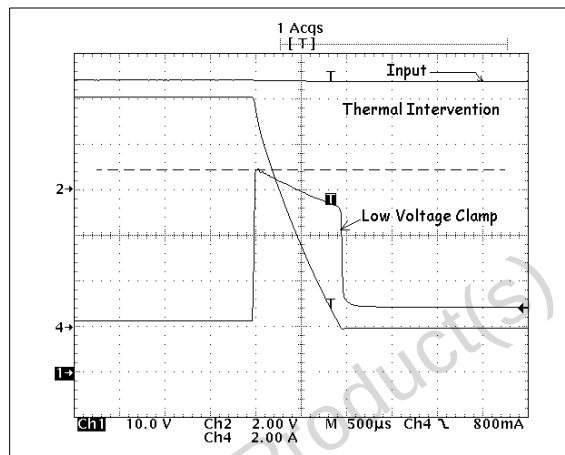
Figure 4: Low voltage clamp feature
