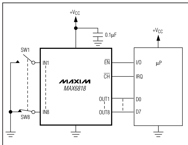
Figure 5. MAX6818 Typical μP Interfacing Circuit
