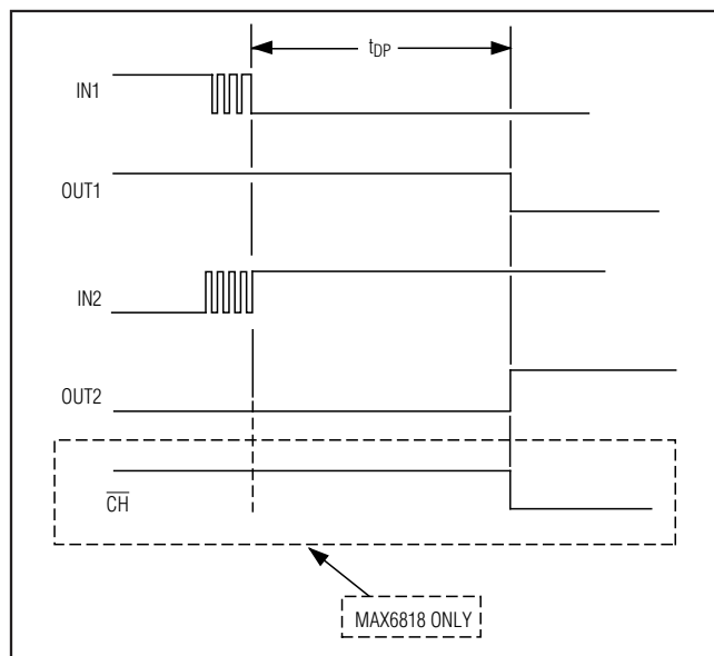
Figure 2. Input Characteristics
